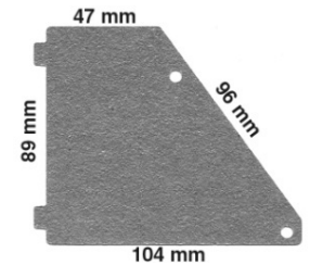
4101 CCE (89X47X96X104MM) MW1300/1350..... 4.30
