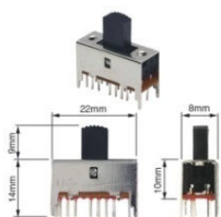
8743 - VERT. 16 TERM.ALAV. 9MM MOD.SS43-D01-G9..... 0.60
